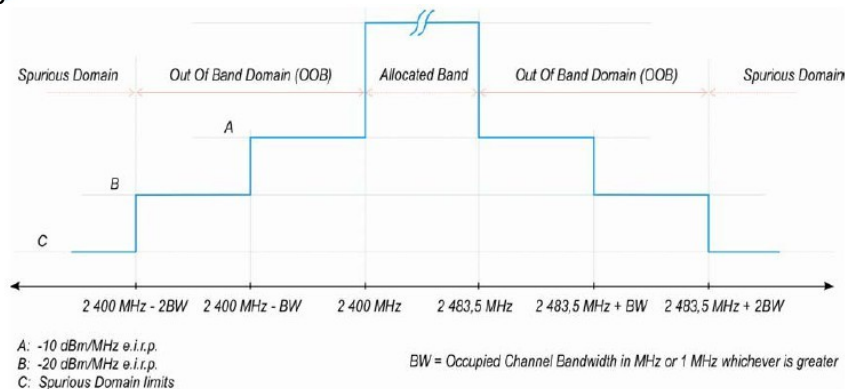
Figure 1: Transmit mask
